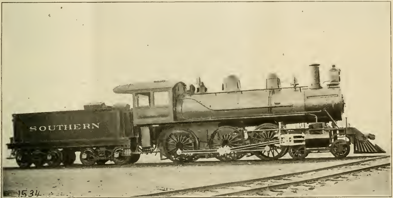
BALDWIN TEN WHEELER FOR THE SOUTHERN.
